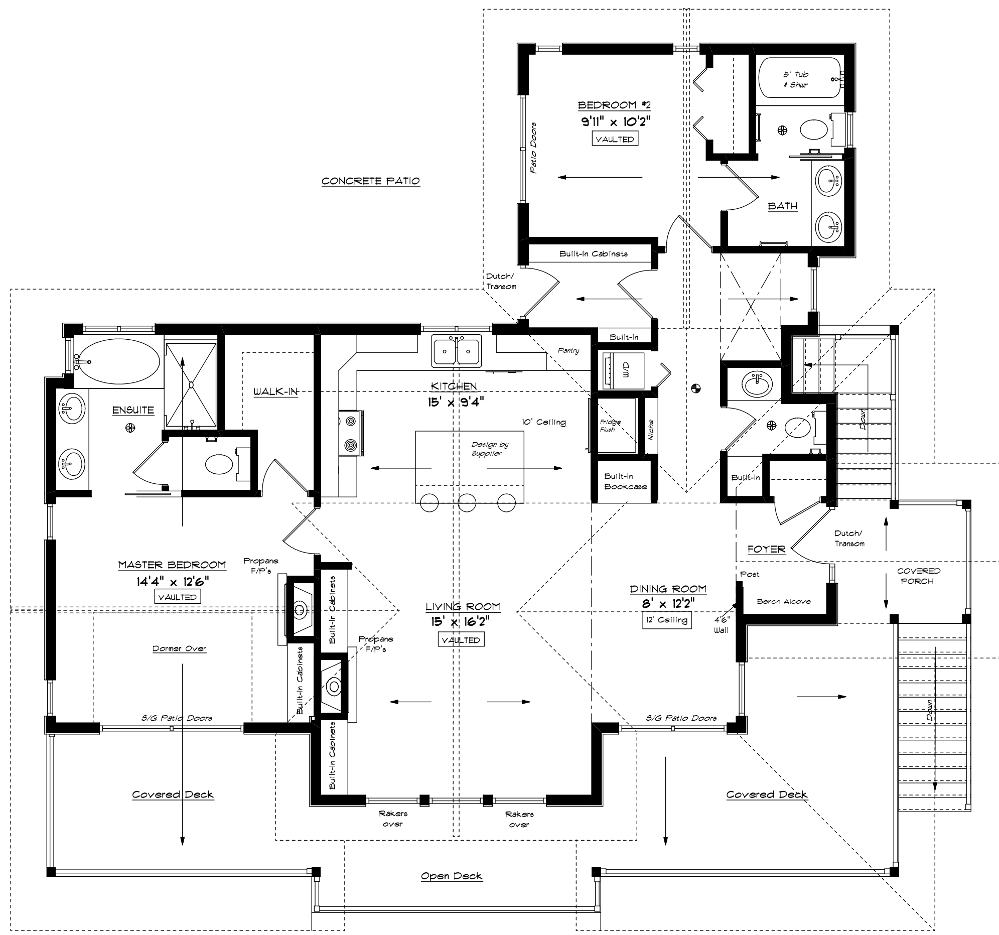
"K2" MAIN FLOOR PLAN 9' 0 3/4" Ceilings 1198 sqFt
