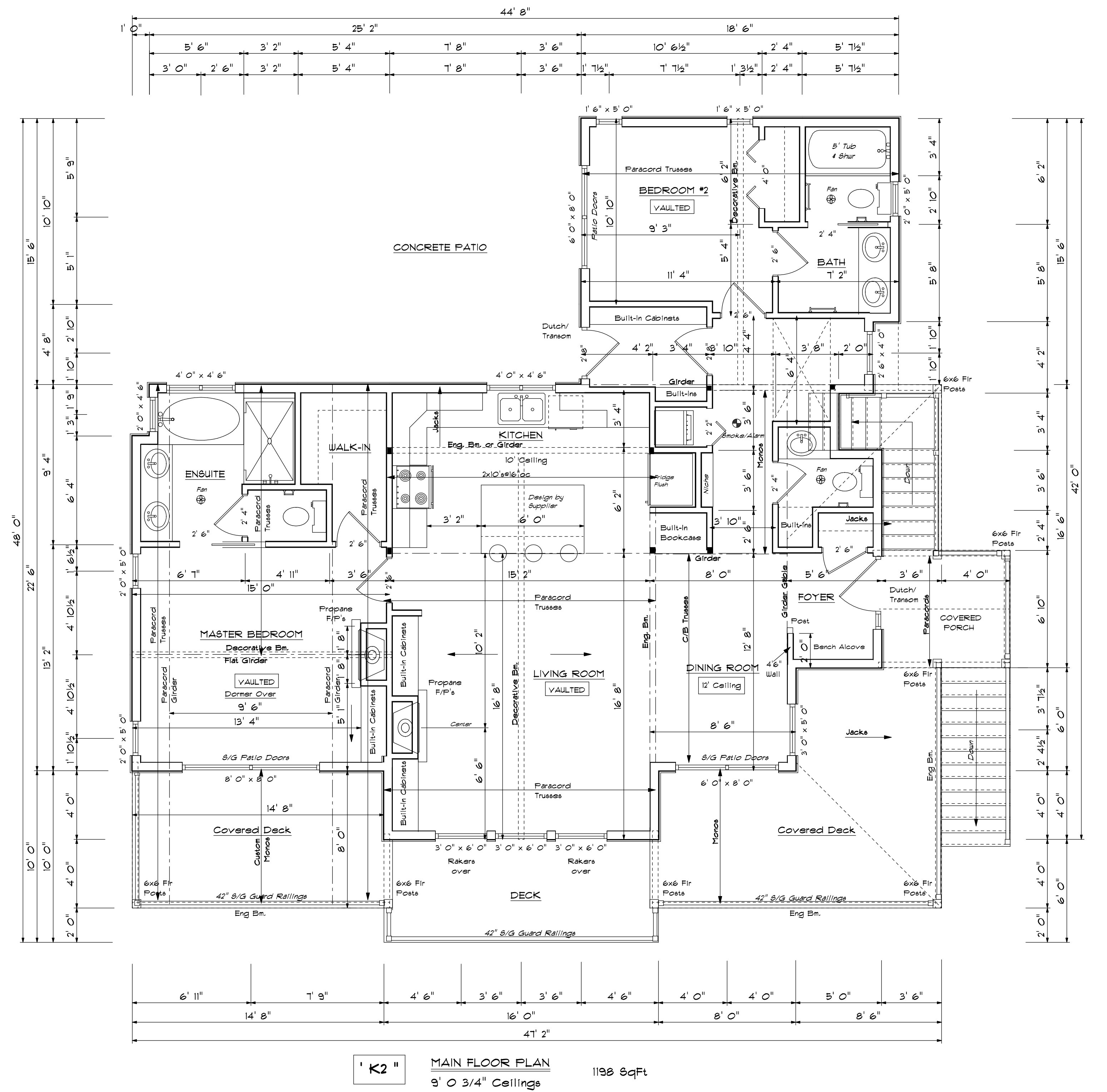
"K2" Option#1 MAIN FLOOR PLAN 9' 0 3/4" Ceilings 1198 sqFt
